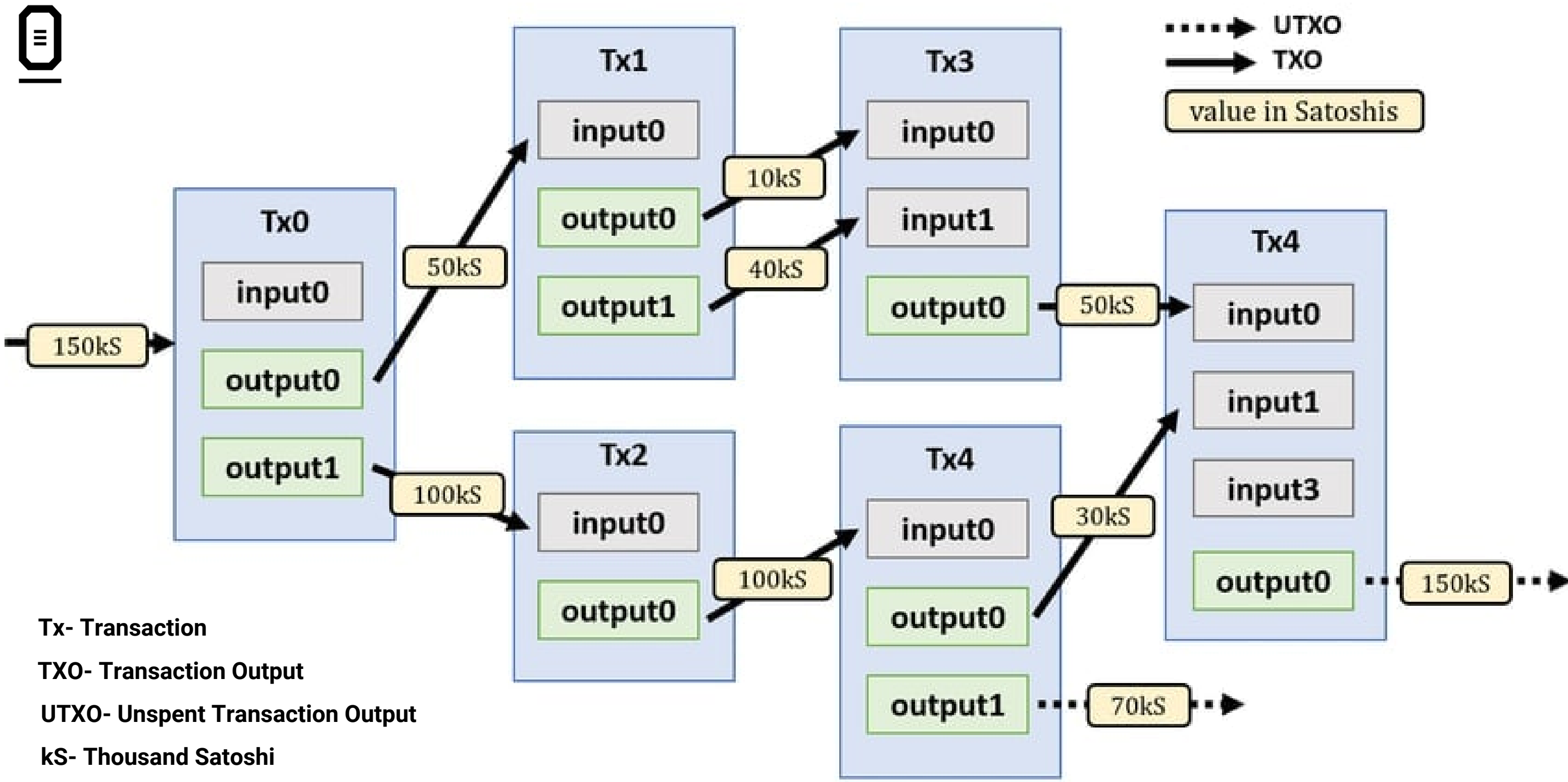
A depiction of UTXO-based transfers in Bitcoin.
